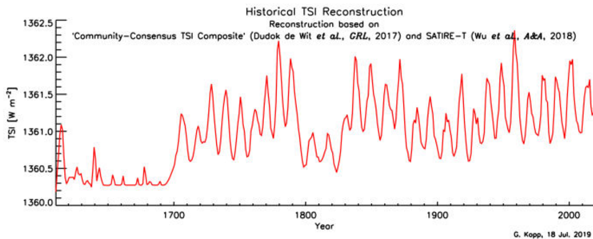
Figure 1. TSI reconstruction 7 by G. Kopp, 2019.
