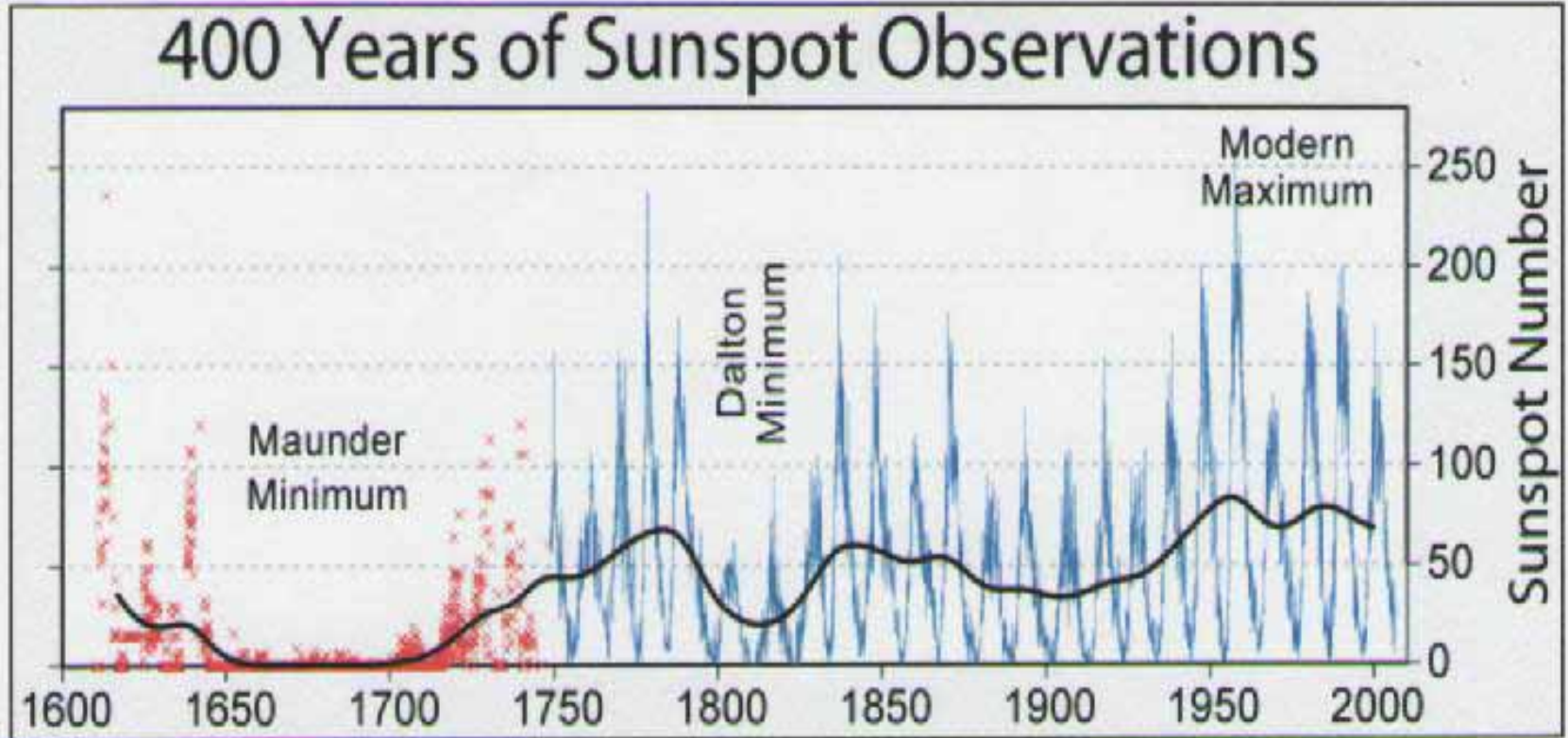
Figure 5.3. 400 Years of Sunspot Numbers with the eleven-year mean of the monthly averages (heavy black line) that shows the Modern Maximum Activity is higher than at any time in the past 400 years shown on the chart (Source, NOAA and Royal Observatory of Belgium, compiled by Hoyt and Schatten, 1998a, 1998b).
