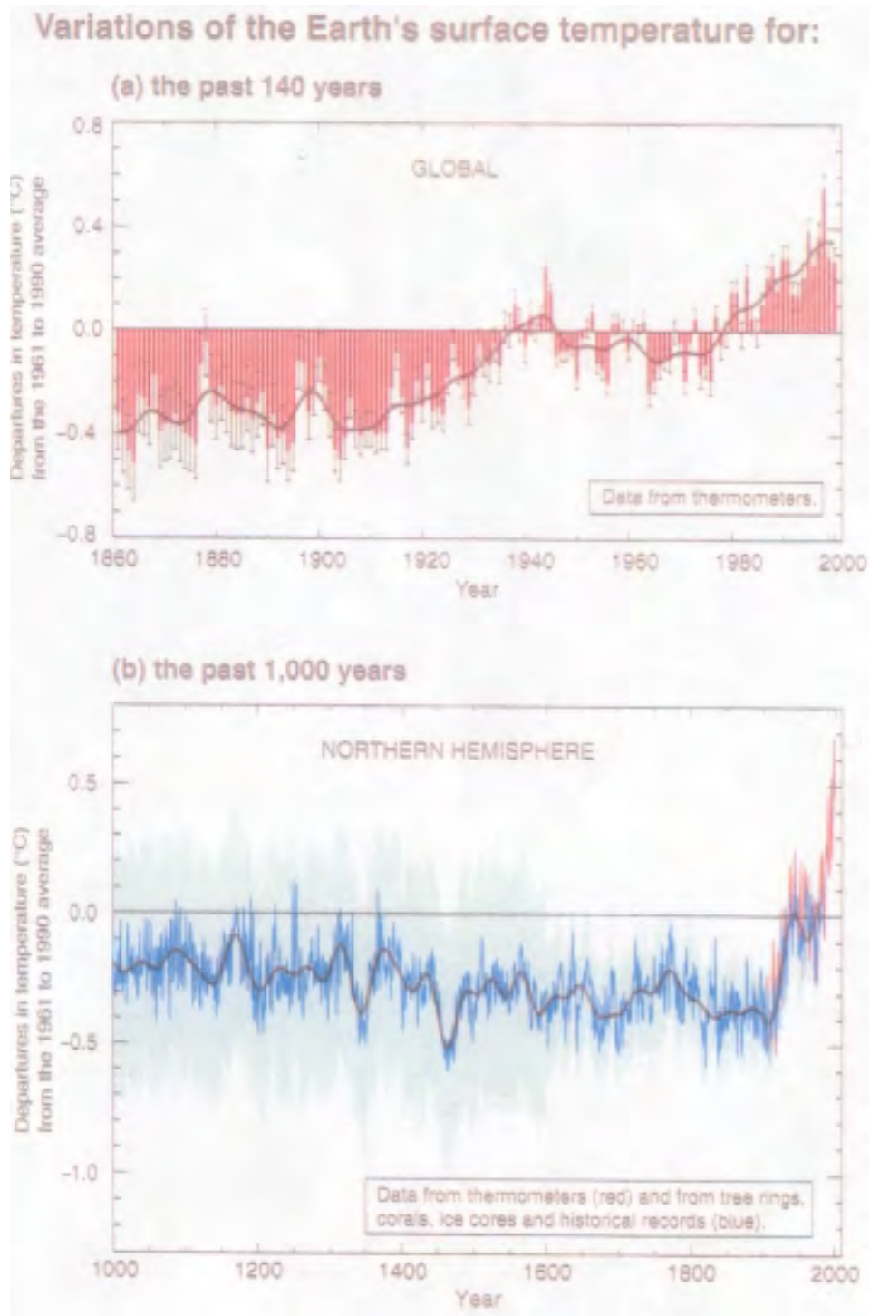
Figure 2.7 Variation of the Earth's surface temperature (a) Global (1860-2000) and (b) Northern Hemisphere (1000-2000) (IPPC, 2001)
