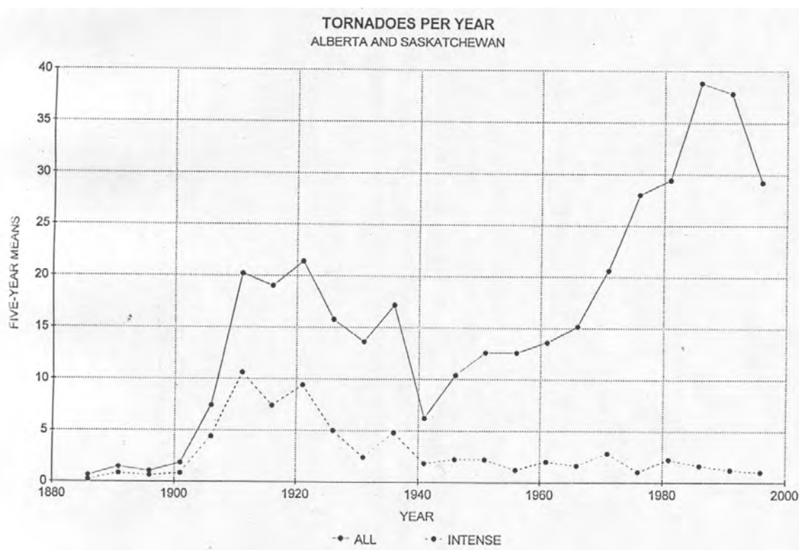
Figure 3.2 Top – Average annual tornado incidence per 10,000 km 2 . Bottom – Five-year averages of annual tornado count for Alberta and Saskatchewan. Data: 1880-1998 (Hage, 2002)
