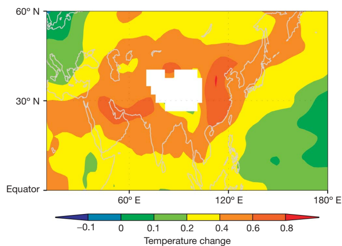
Figure 3 | The temperature change dT due to ABC solar heating at the 700 hPa (or 700 mb) level ( \sim 3 km a.s.l.) simulated by CCM3. The change is estimated from a 50-year average of experiment and control. The standard error of the mean difference is 0.05 K. All altitudes mentioned in the text are a.s.l. altitudes. For example, a warming of 0.6 K at 3 km a.s.l. would denote near-surface warming for a location in the Himalayas that is at an elevation of 3 km a.s.l. The white-shaded regions are the part of the Himalayas with surface pressure less than 700 mb, that is, surface elevations are higher than 3 km.
