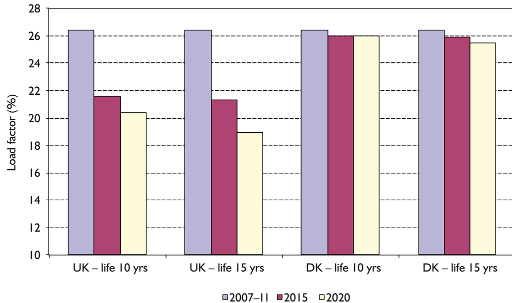
Figure 6A: Projected load factors for UK onshore wind (total capacity of 10 GW in 2020)
